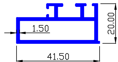
SEC. NO.-90220 WT.-0.541 Kg/Mtr.
