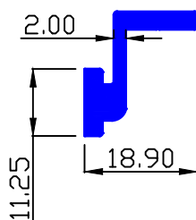
SEC. NO.-90228 WT.-0.314 Kg/Mtr.
